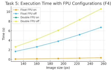
Fig. 4. Execution times with FPU configurations
