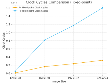
Fig. 2. Clock cycles comparison
