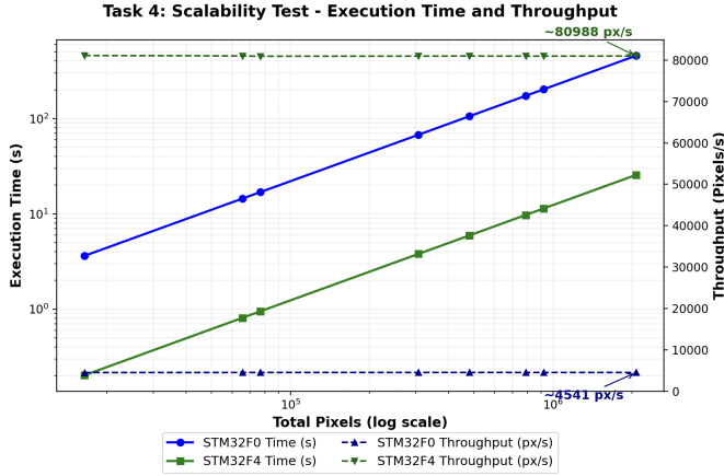
Fig. 3. Scalability analysis showing execution time and computational throughput for the STM32F0 and STM32F4
